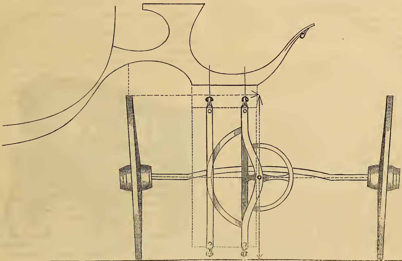
DIAGRAM FOR DETERMINING THE PROPER PLACE FOR THE KING-BOLT.
